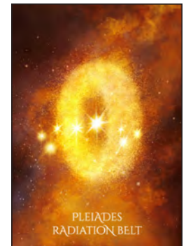
Pleiades Radiation Belt
